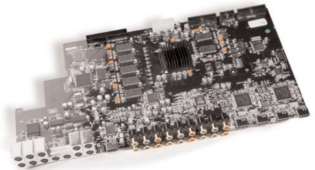
6-layer digital video processing board with gold traces and over 1,800 parts, the same one used in the critically acclaimed Anthem™ Statement D2
